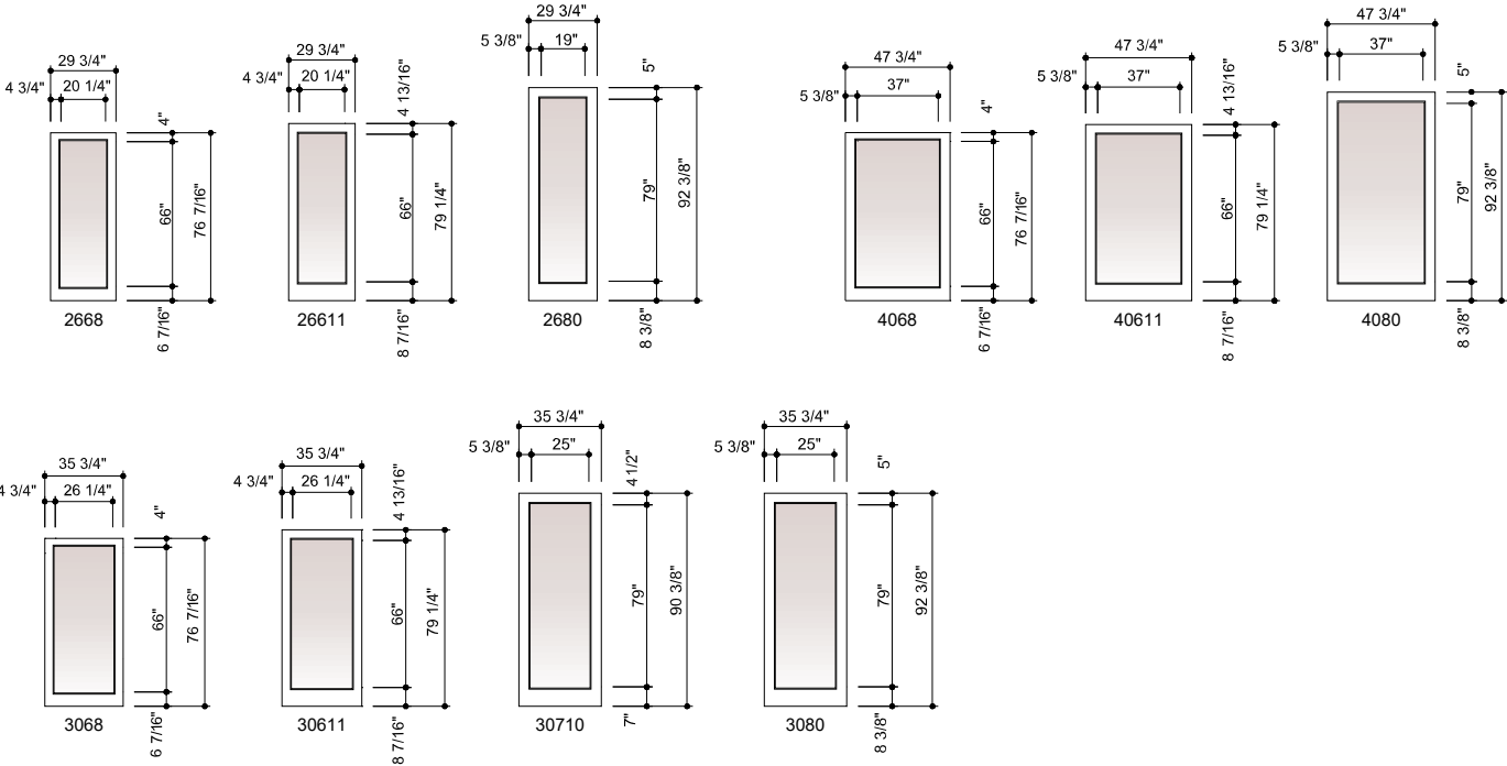
Gliding Patio Doors - 3/4 Lite
