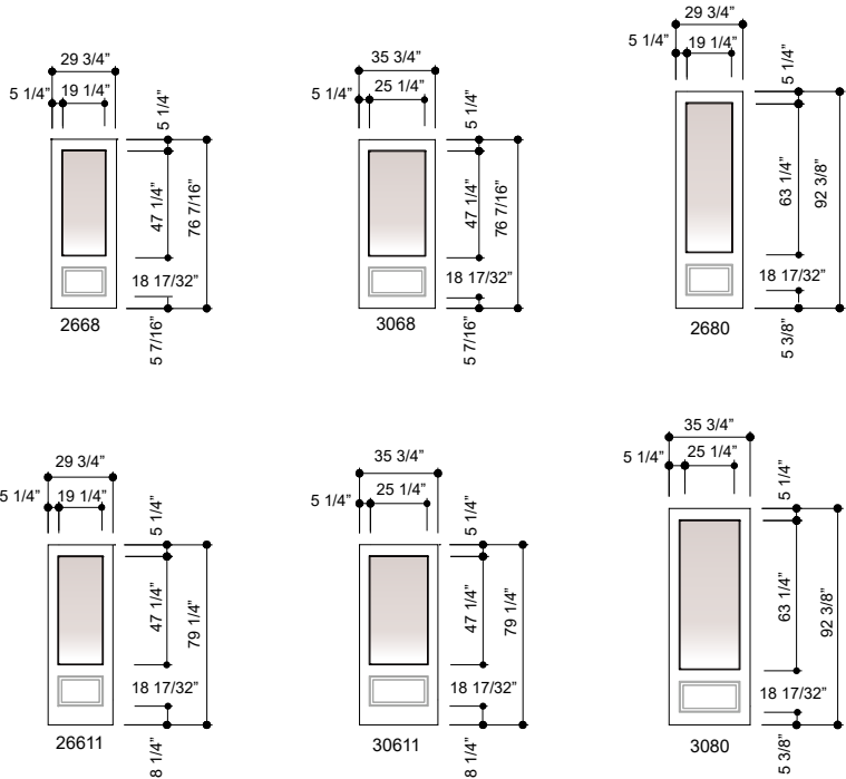
Gliding Patio Doors - 3/4 Lite
